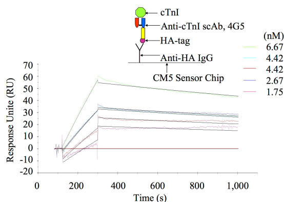
Fig. 2 Kinetic analysis of interactions between anti-cTnI scAb and cTnI using the Biacore 3000 system
