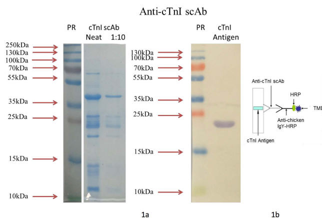
Fig. 1 SDS-PAGE and Western blotting analysis of purified anti-cTnI scAb
